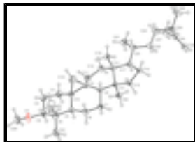
Fig. 1. ORTEP-3 (Farrugia, 1997) drawing of (I) with displacement ellipsoids plotted at 30% probability level.
